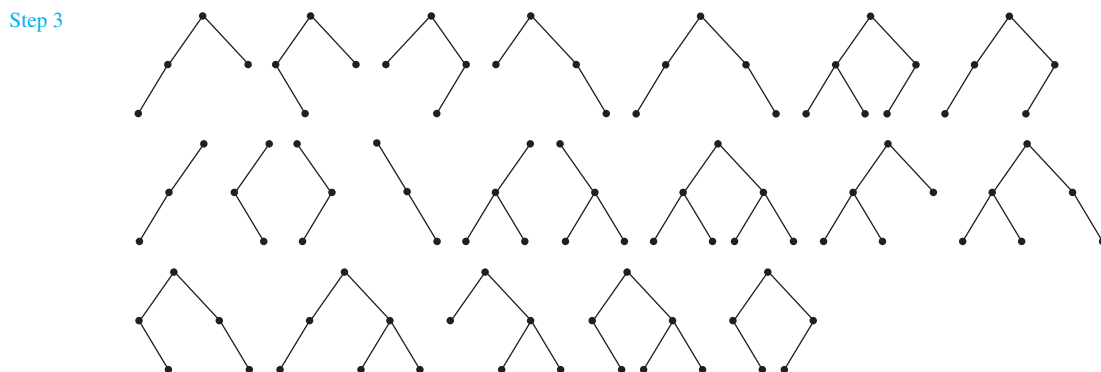
FIGURE 3 Building Up Extended Binary Trees.
