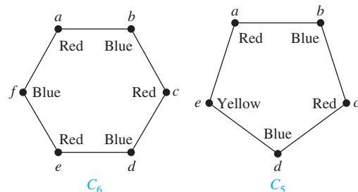
FIGURE 7 Colorings of C_5 and C_6 .
